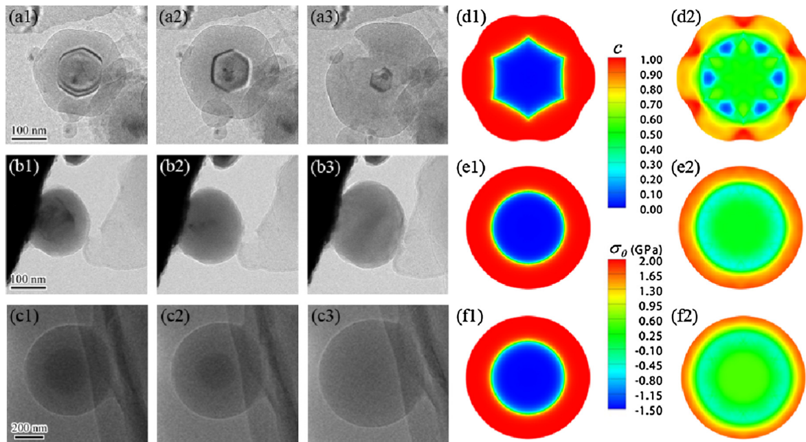
Fig. 14. Lithiation-induced anisotropic swelling and fracture in a c -SiNP versus the isotropic swelling without fracture in a c -GeNP and an a -SiNP. The original sizes of the c -SiNP and c -GeNP are both about 160 nm, and the a -SiNP is about 540 nm. (a1–a3) TEM image sequence showing the anisotropic swelling and subsequent fracture of a lithiated c -SiNP [34]. The round c -SiNP becomes hexagonal in shape for both the outer surface and inner unlithiated core. (d1–d2) Chemo-mechanical modeling of the core-shell structure and stress generation in the cross section of a lithiated c -SiNP [80]. The red color at the outer surface indicates tensile stress, while the blue color indicates compressive stress. (b1–b3) TEM image sequence shows the isotropic swelling and tough behavior of c -GeNP [34]. (e1 and e2) Chemo-mechanical modeling of the uniform stress generation in the cross section of a lithiated amorphous c -GeNW [80]. (c1–c3) TEM image sequence shows the isotropic swelling and tough behavior of a -SiNP [134]. (f1 and f2) Chemo-mechanical modeling of the uniform stress generation in the cross section of a lithiated a -SiNW [80].
