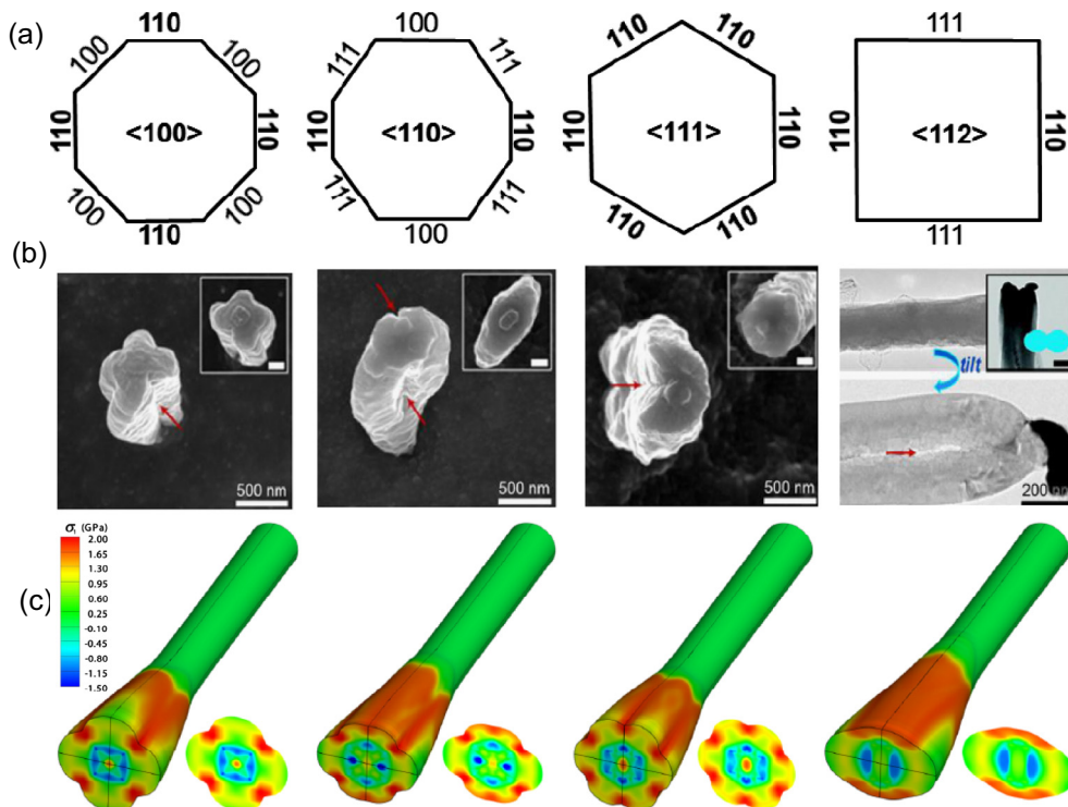
Fig. 9. (a) Lithiation-induced fracture of four c\text{-SiNW} s with different crystallographic orientations. Indices in the center represent the axial orientation, while those on the sides represent the orientations of the facets. (b) SEM (the first three columns) [32,34] and TEM (the last column) [43] images showing the crack nucleation sites (marked by red arrows) in the lithiated c\text{-SiNW} s of four different orientations. (c) The experimentally observed crack nucleation sites coincide with the stress concentration locations (red spots) predicted by the front-tracking finite element modeling [115].
