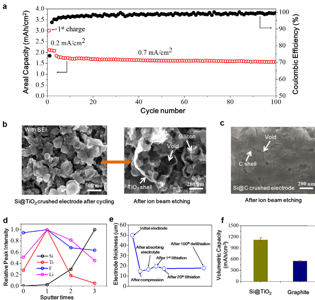
Fig. 5. Crushed \text{Si@TiO}_2 electrode vs \text{Si@C} electrode. (a) Full-cell performance of crushed \text{Si@TiO}_2 cluster anode ( 2.1\text{ mg/cm}^2 ) paired with commercial 3\text{ mA h/cm}^2 \text{LiCoO}_2 cathode. (b) SEM image of \text{Si@TiO}_2 crushed electrode ( 30\text{ MPa} ) after 100 cycles (full cell). Left part is with SEI and right part is after ion beam etching. (c) SEM image of \text{Si@C} crushed electrode ( 30\text{ MPa} ) after 50 cycles. (d) Relative peak intensity (Si, Ti, F, and Li) of \text{Si@TiO}_2 cluster electrode after 1500 cycles discharging and charging measured by X-ray photoelectron spectroscopy (XPS) during 3 ion sputtering times. Time 0 means before sputter. (e) Electrode thickness variation. (f) Volumetric specific capacity of \text{Si@TiO}_2 vs. commercial graphite. Taken from [65].
