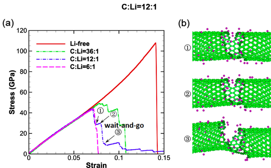
Fig. 11. Li concentration dependent fracture behavior of SWCNTs [159]. (a) Stress-strain curves of SWCNTs with different Li concentrations. For intermediate Li concentrations, the crack propagates in a “wait-and-go” manner. (b) The three representative atomic configurations of the SWCNT (Li: C = 1:12) on the “wait-and-go” fracture path, indicated in (a).
